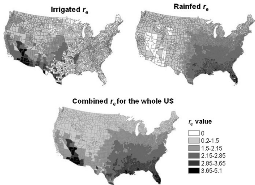
Fig. 6 External influence coefficient ( r_e ) estimated from irrigated ( top left ), rainfed ( top right ), and area weighted average (using combined rainfed and irrigated areas; bottom ) for the US counties
